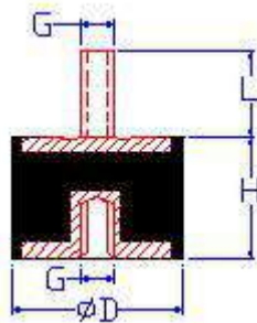
Footprint dimensions for vertical/horizontal mounting[mm]
